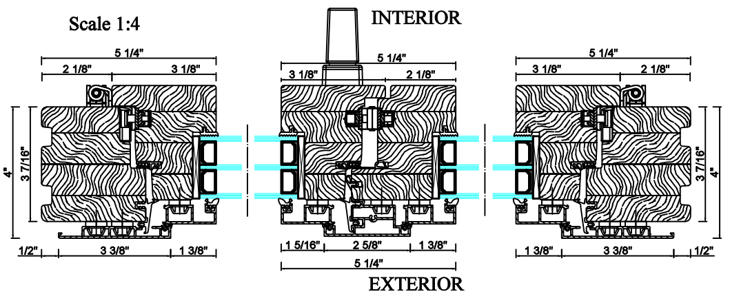
Horizontal cross section A-A
