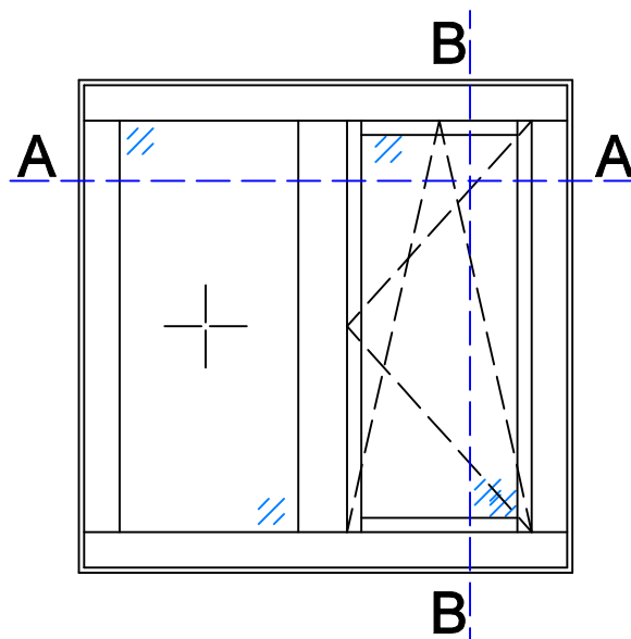
Windows type: FIX + Tilt&Turn
