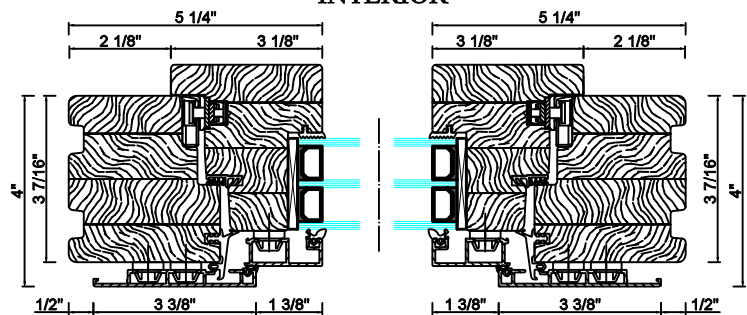
Horizontal cross section A-A
