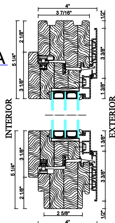
Windows type: FIX + Tilt&Turn
