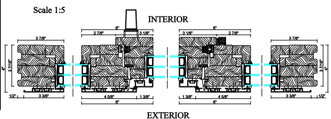
Horizontal cross section A-A
