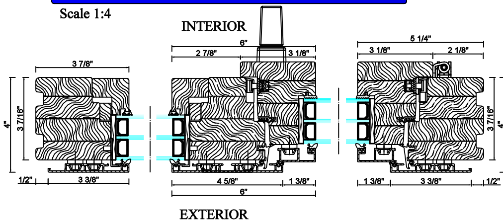
Horizontal cross section A-A
