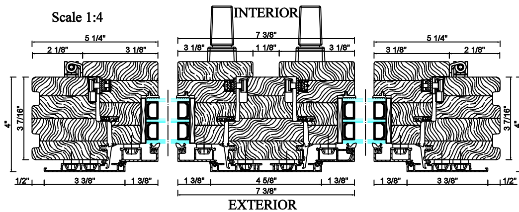
Horizontal cross section A-A
