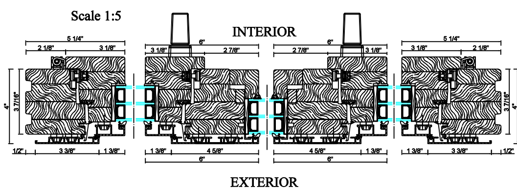
Horizontal cross section A-A
