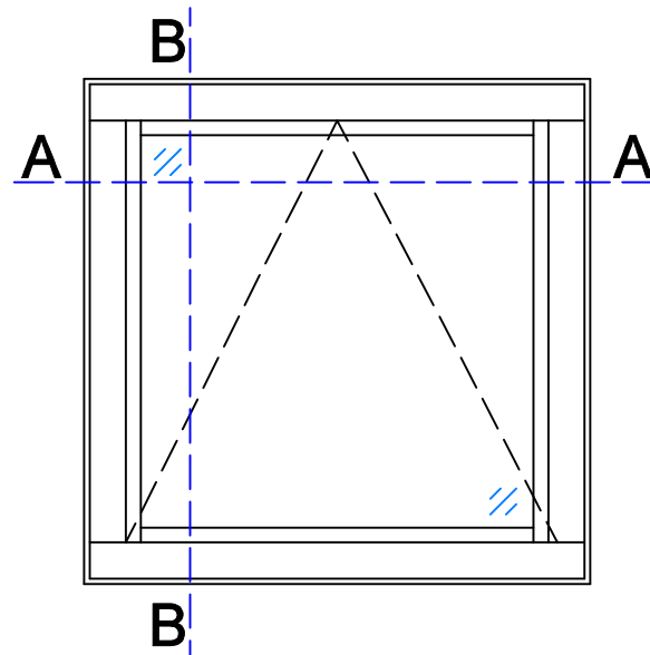
Windows type: Tilt
