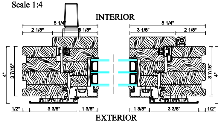
Vertical cross section B-B
